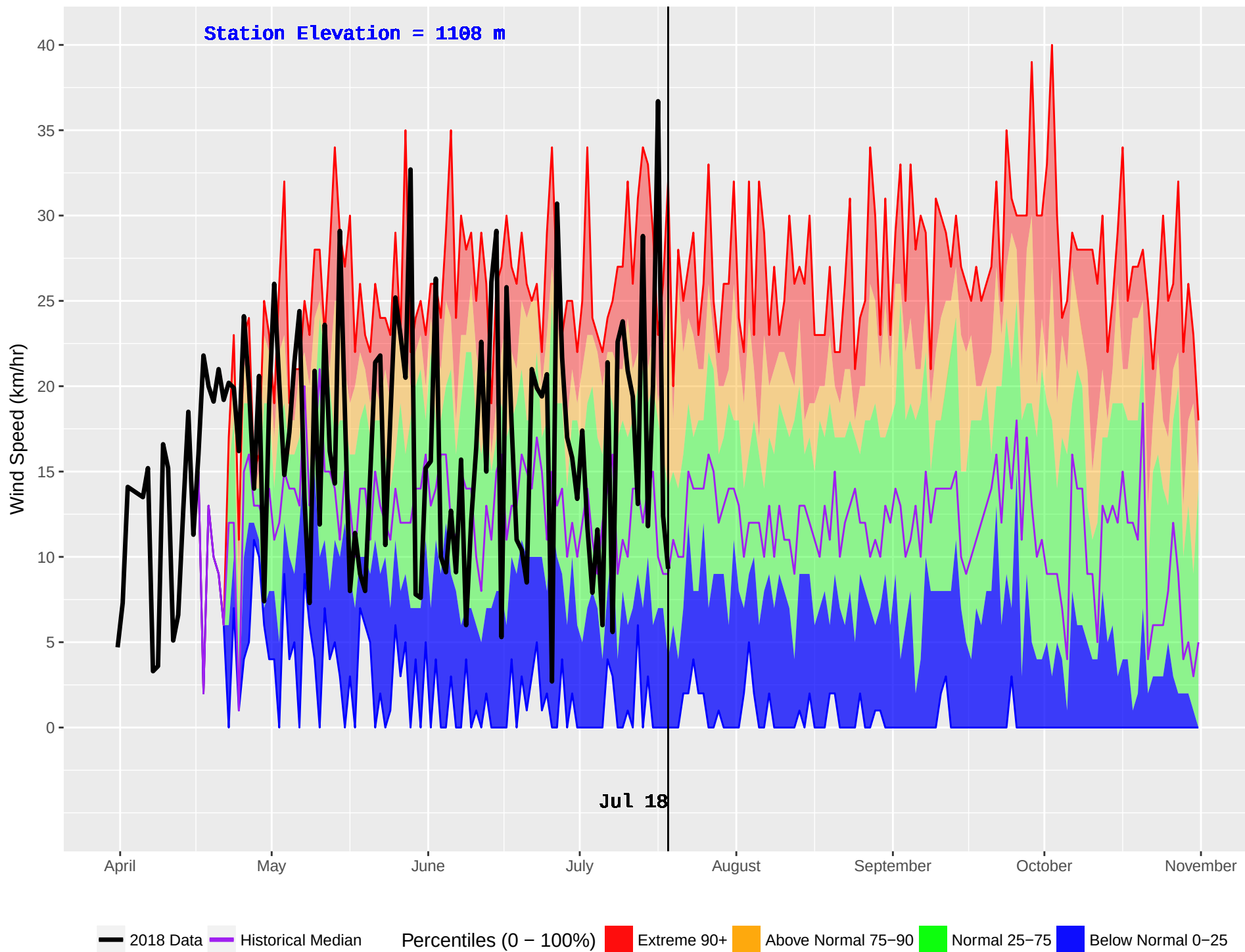
NABESHE (151) : Historical (1987–2016) and Current (2018) Daily Wind Speed
