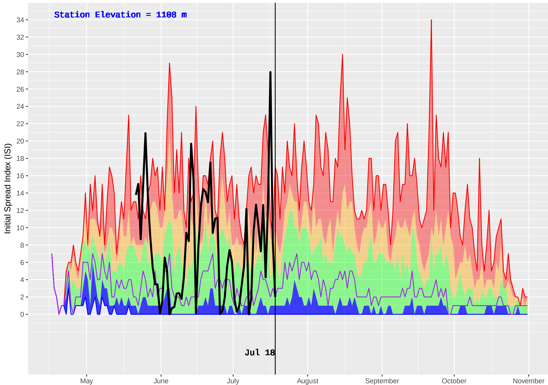
NABESHE (151) : Historical (1987–2016) and Current (2018) Daily Initial Spread Index (ISI)
