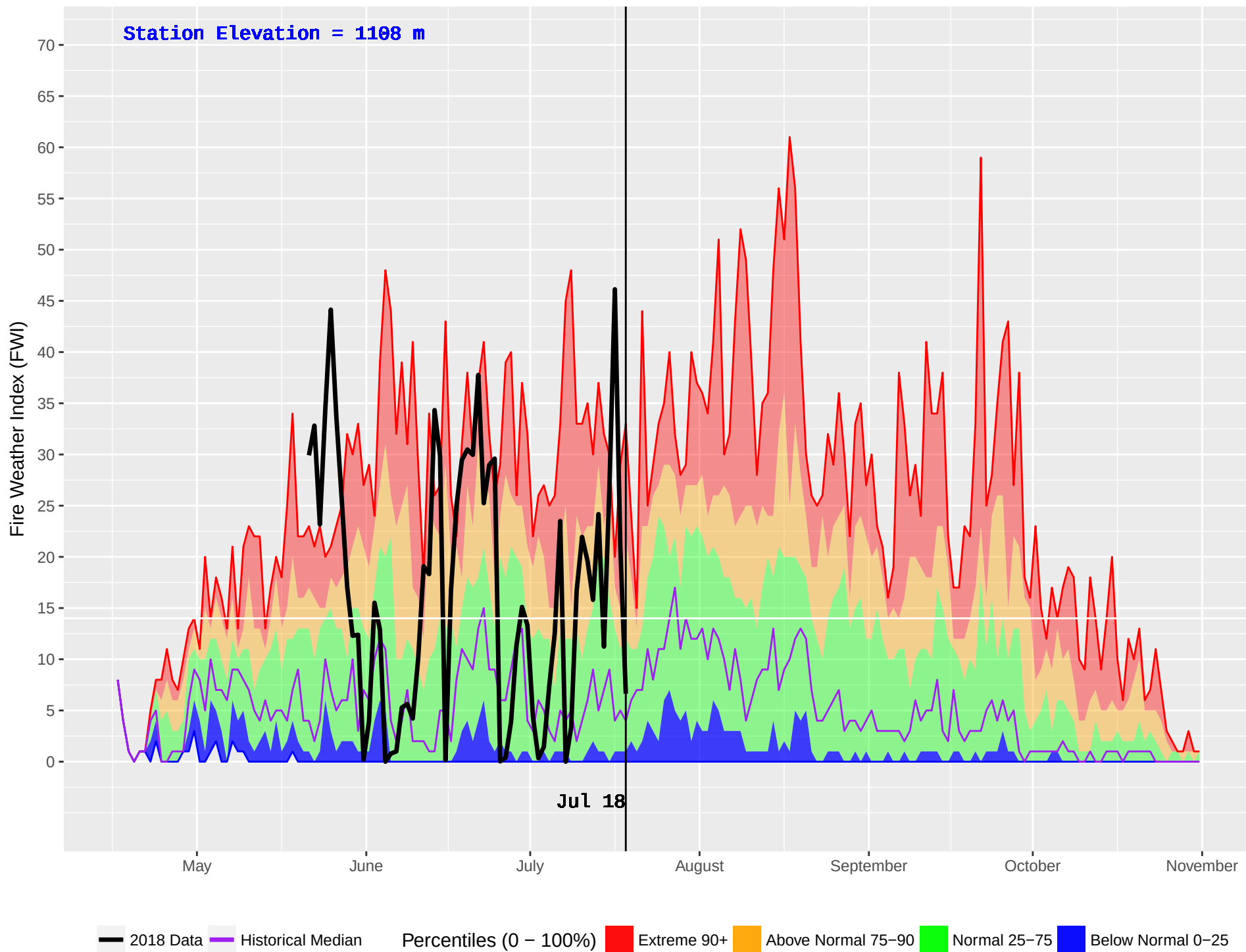
NABESHE (151) : Historical (1987–2016) and Current (2018) Daily Fire Weather Index (FWI)
