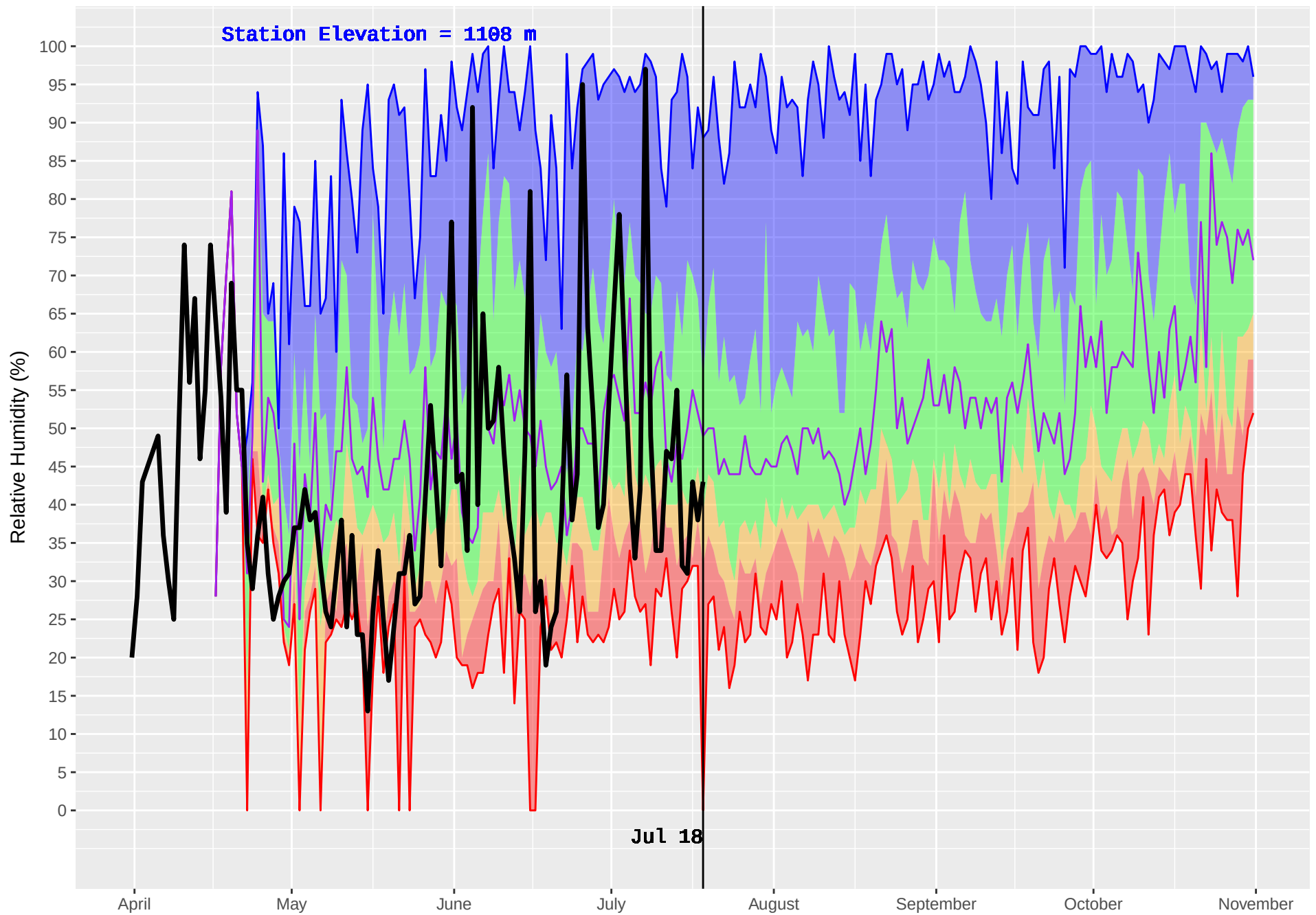
NABESHE (151) : Historical (1987–2016) and Current (2018) Daily Relative Humidity
