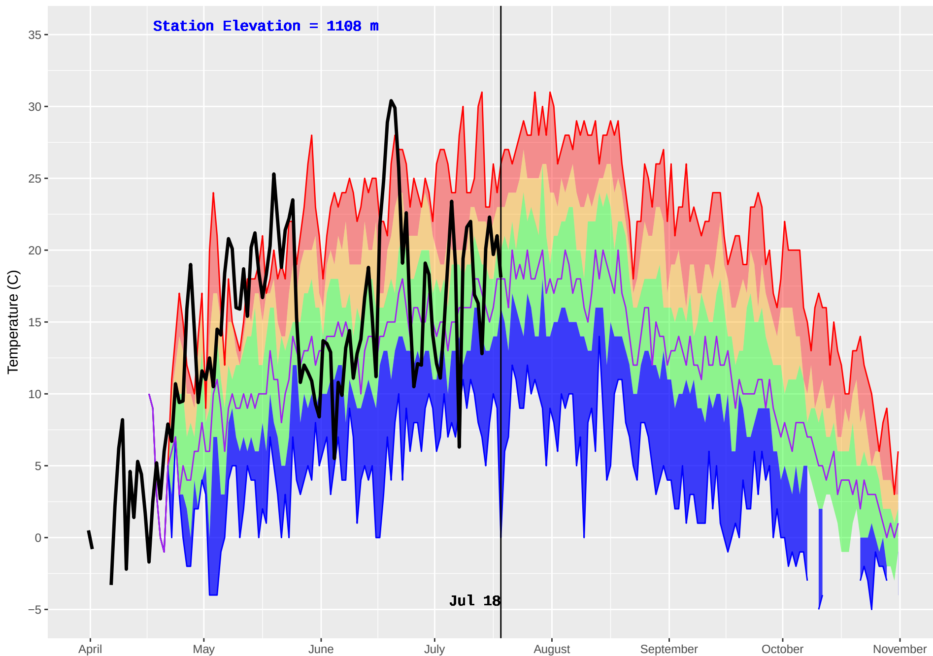
NABESHE (151) : Historical (1987–2016) and Current (2018) Daily Temperature
