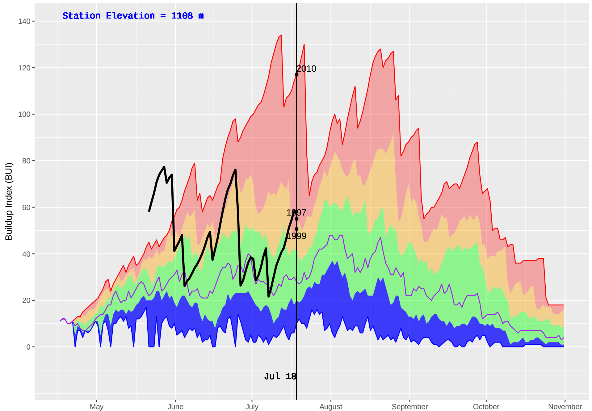
NABESHE (151) : Historical (1987–2016) and Current (2018) Daily Buildup Index (BUI)
