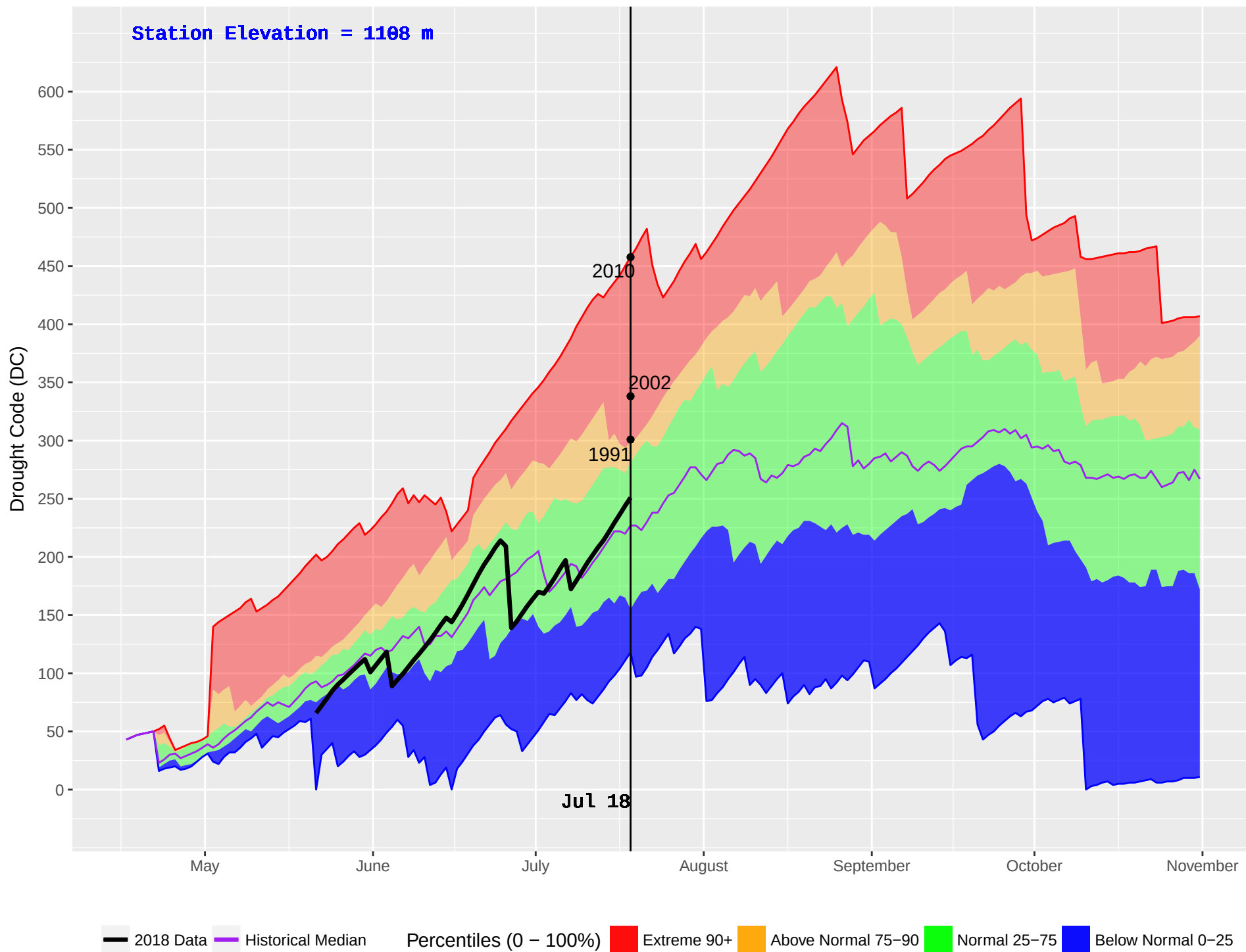
NABESHE (151) : Historical (1987–2016) and Current (2018) Daily Drought Code (DC)
